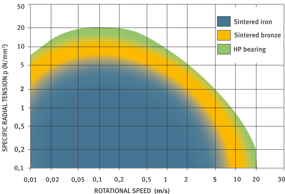
Critical load diagram for sintered bearings
