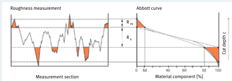
Abbott curve measured in accordance with DIN EN 13565.
