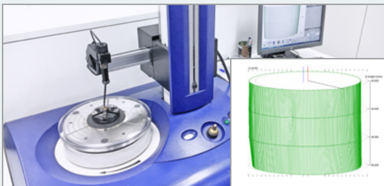
Apparatus to measure cylindrical form
