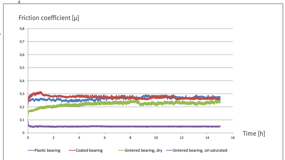
Friction coefficients of various bearing types
